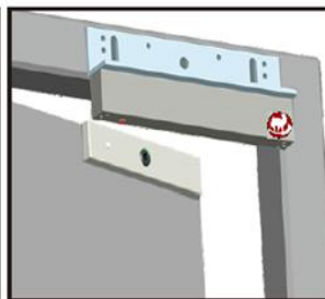
Demonstration of L Bracket Installation
